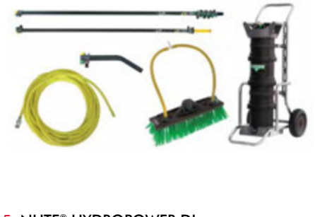
5. NLITE® HYDROPOWER DI PROFESSIONAL KIT nLite® HydroPower DI PROFESSIONAL KIT; Content: DI48C nLite HydroPower DI 24 L · CT67G nLite Carbon Fibre Master Pole 6.63 m · CT35G nLite Carbon Fibre Extension Pole 3.41 m · NLG20 nLite MultiLink Angle Adapter 20 cm · NLR27 nLite Radius Brush 27 cm · NL25G nLite Hose 25 m
